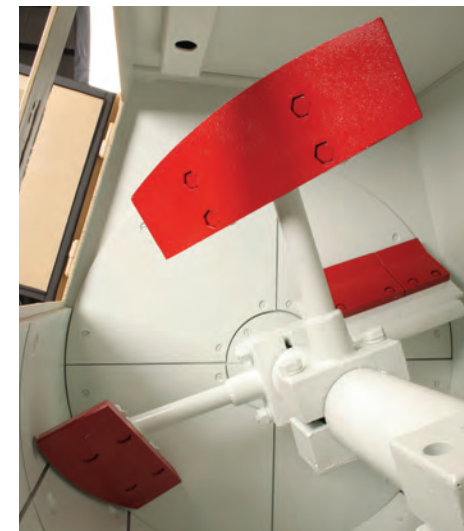
Cast Ni-Hard mixing paddles resist abrasion and are easily replaceable*
