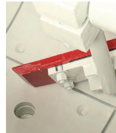
Cast Ni-Hard liner segments bolted in for easy replacement*
