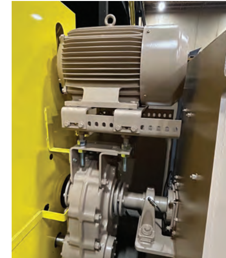
Shaft mounted mixer drive with oil-bath lubricated gear box for long life
