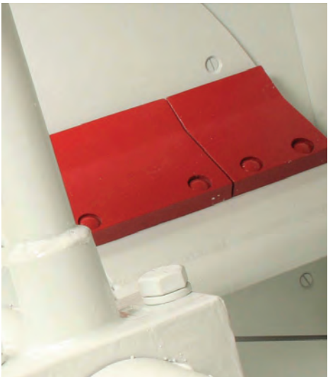
Cast Ni-Hard wall scraper blades resist wear*
