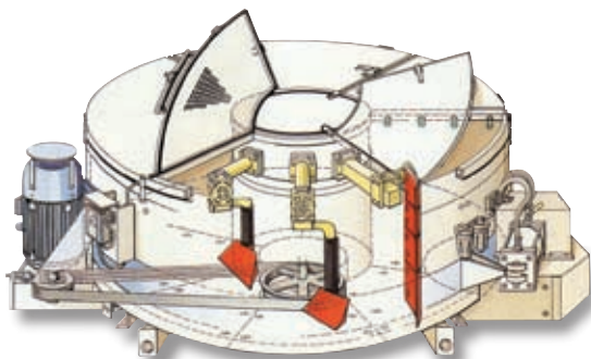
Cut-away view showing belt drive of transmission
